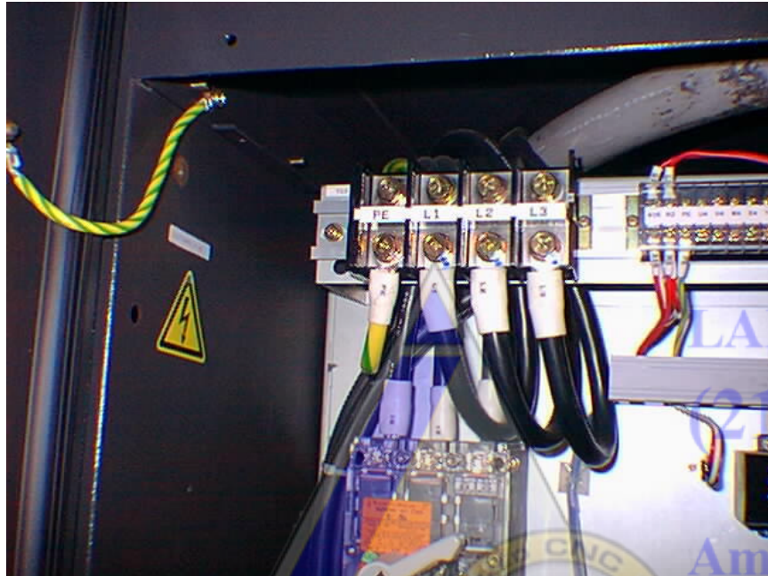
Vipros 357 Queen rear of electrical enclosure
