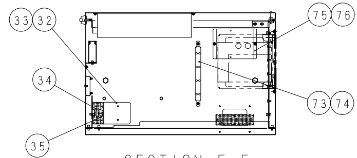
SECTION F-F
